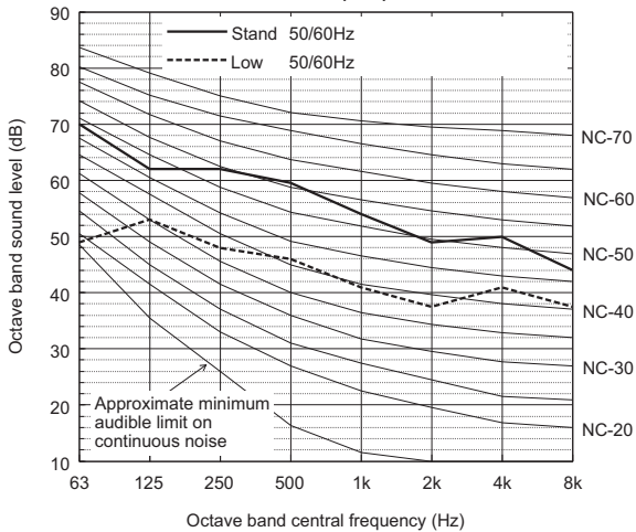
Sound level of PUHY-EP250YNW-A(-BS)
