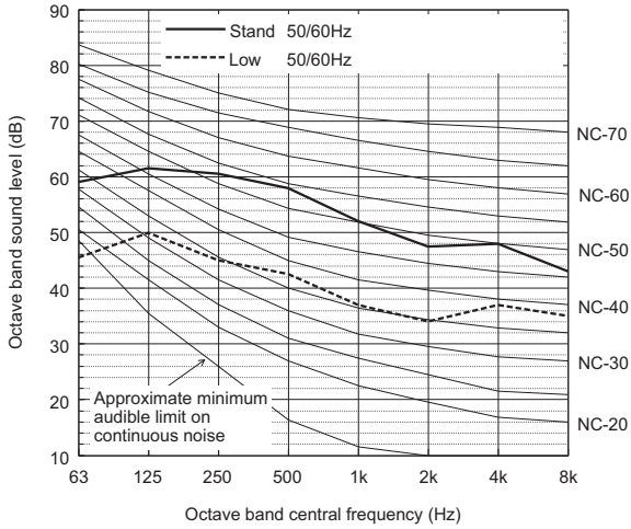
Sound level of PUHY-EP200YNW-A(-BS)
