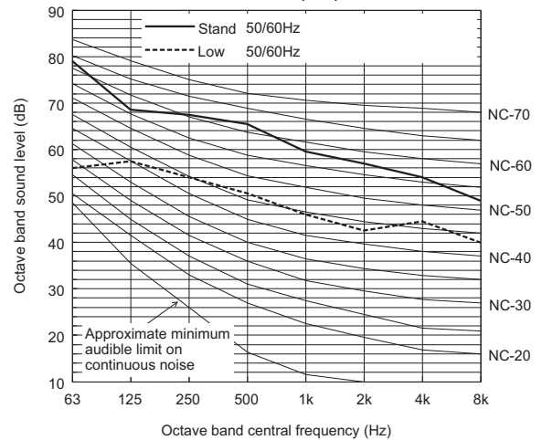
Sound level of PUHY-EP650YSNW-A(-BS)
