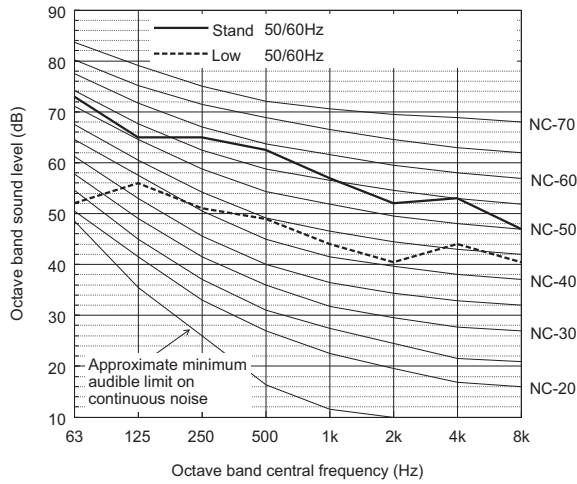
Sound level of PUHY-EP500YSNW-A(-BS)
