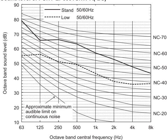
Sound level of PUHY-EP600YSNW-A(-BS)
