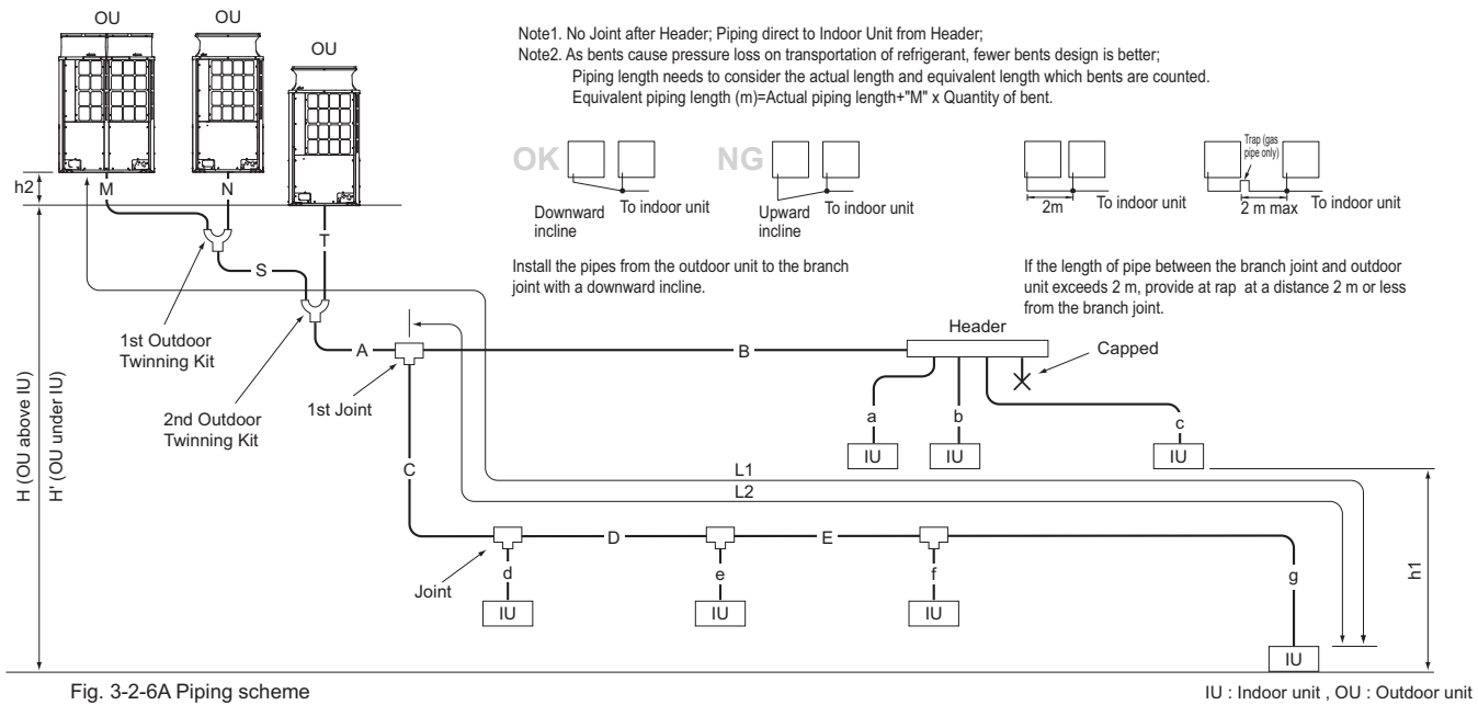
Fig. 3-2-6A Piping scheme
