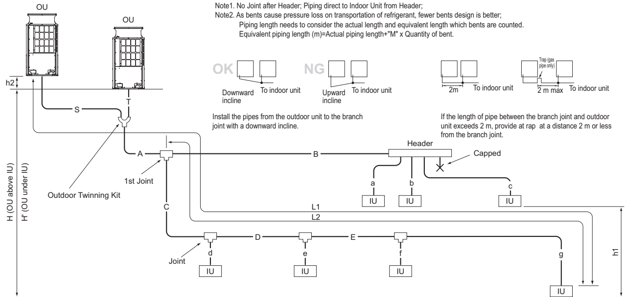
Fig. 12-2-2A Piping scheme
