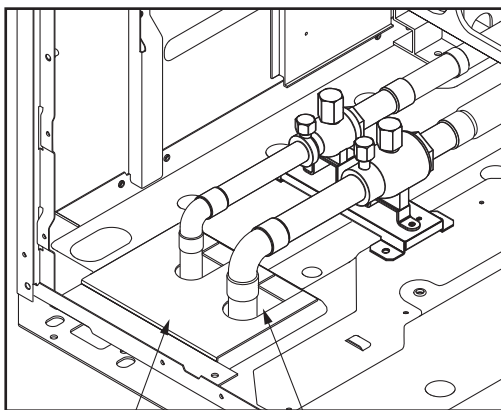
Example of closure materials (field supply) Fill the gap at the site (field supply)
