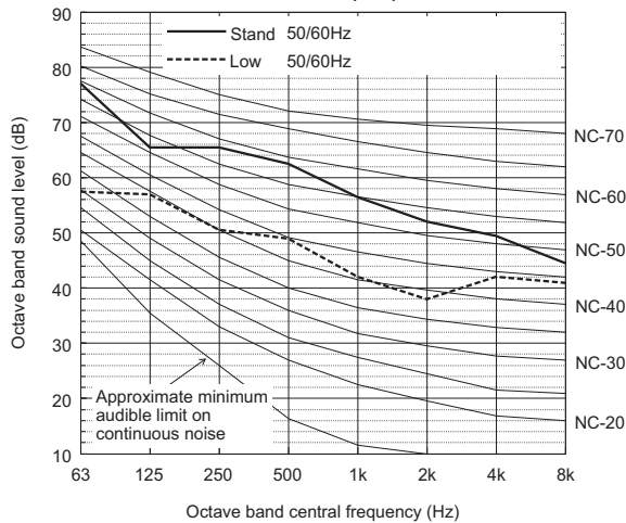
Sound level of PUHY-EP550YSNW-A(-BS)
