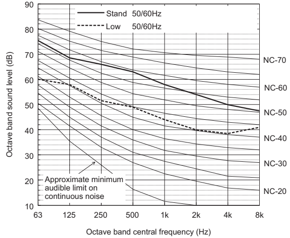
Sound level of PUHY-EP300YNW-A(-BS)
